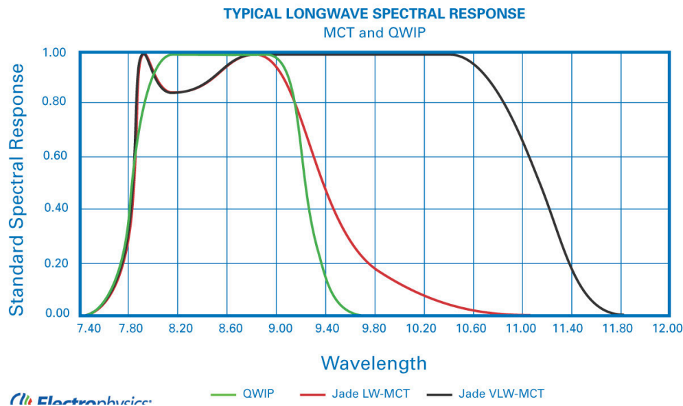
Figure 1: Normalized Spectral Response for Qwip, LW-MCT and VLW-MCT
